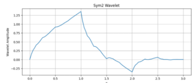
Figure 3: Symlet Wavelets
