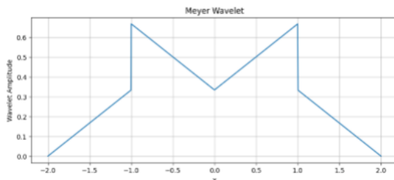
Figure 5: Meyer Wavelets
